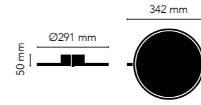
INLAY ROUND C2 18W LED - 220-240V
