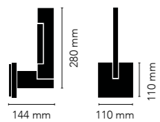
INLAY W1 6W LED - 220-240V
