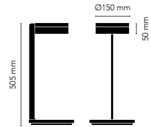
BLADE T2 SLIM 12.5W LED - 220-240V
