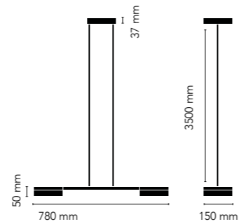
BLADE S2 SLIM 2x16W LED - 220-240V
