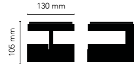
BLADE C1+ SLIM 13.3W LED - 220-240V
