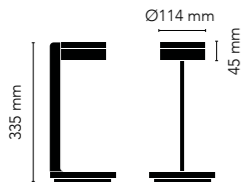
BLADE T1 SLIM 9W LED - 220-240V
