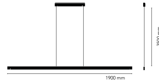
INLAY S1900 38W LED - 220-240V
