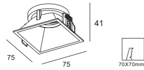
DH0089 Gu10/Mr16 Downlight Cutout :70X70mm Optional :ALDL1401 ALDL1373 ALDL1022
