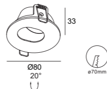
DH0105 Gu10/Mr16 Downlight Cutout :ø70mm Optional :ALDL1401 ALDL1373
