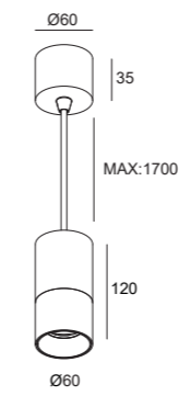
TR0073 Gu 10 Track Light
