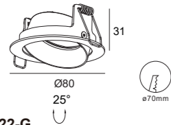
DL0122-G Gu10/Mr16 Downlight Cutout :ø70mm Optional :ALDL1401 ALDL1373
