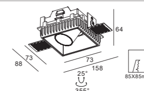
DH0058 Gu10/Mr16 Downlight Cutout :85x85mm Optional :ALDL1401 ALDL1373 ALDL1022
