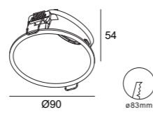
DH0110 Gu10/Mr16 Downlight Cutout :Ø83mm Optional :ALDL1401 ALDL1373 ALDL1022
