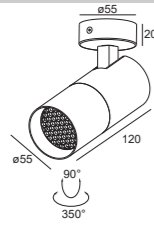
CH0131 Gu 10 Ceiling Surface Light
