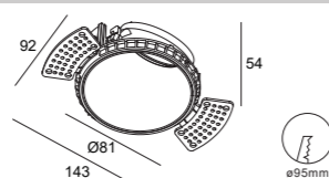
DH0111 Gu10/Mr16 Downlight Cutout :Ø95mm Optional :ALDL1401 ALDL1373 ALDL1022
