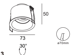
DH0113 Gu10/Mr16 Downlight Cutout :Ø70mm Optional :ALDL1401 ALDL1373 ALDL1022
