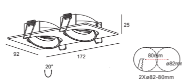
DL0031-G Gu10/Mr16 Downlight Cutout :2Xø82-80mm Optional :ALDL1401 ALDL1373
