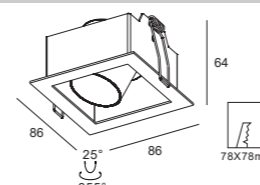
DH0054 Gu10/Mr16 Downlight Cutout :78x78mm Optional :ALDL1401 ALDL1373 ALDL1022
