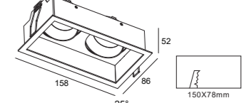
DH0050 Gu10/Mr16 Downlight Cutout :150X78mm Optional :ALDL1401 ALDL1373 ALDL1022
