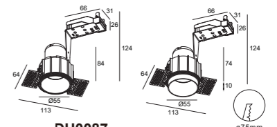
DH0087 E27 Downlight Cutout :ø75mm
