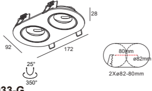
DL0033-G Gu10/Mr16 Downlight Cutout :2Xø82-80mm Optional :ALDL1401 ALDL1373
