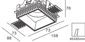
DL0176-G Gu10/Mr16 Downlight Cutout :85X85mm Optional :ALDL1401 ALDL1373 ALDL1022
