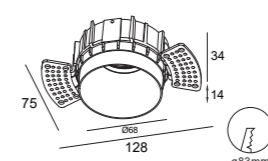
DH0088 Gu10/Mr16 Downlight Cutout :ø83mm Optional :ALDL1401 ALDL1373 ALDL1022
