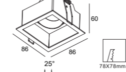
DH0112 Gu10/Mr16 Downlight Cutout :150X78mm Optional :ALDL1401 ALDL1373 ALDL1022
