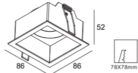
DL0014-G Gu10/Mr16 Downlight Cutout :78X78mm Optional :ALDL1401 ALDL1373 ALDL1022
