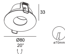
DH0104 Gu10/Mr16 Downlight Cutout :ø70mm Optional :ALDL1401 ALDL1373
