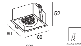
DH0091 Gu10/Mr16 Downlight Cutout :75X75mm
