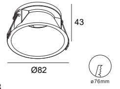
DH0048 Gu10/Mr16 Downlight Cutout :ø76mm Optional :ALDL1401 ALDL1373 ALDL1022
