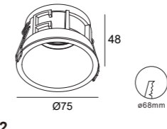
DH0092 Gu10/Mr16 Downlight Cutout :ø68mm Optional :ALDL1401 ALDL1373 ALDL1022
