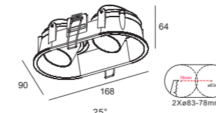
DH0053 Gu10/Mr16 Downlight Cutout :2xØ83-78mm Optional :ALDL1401 ALDL1373 ALDL1022
