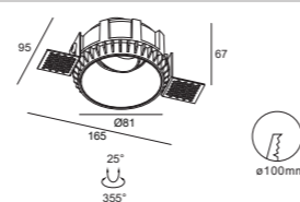
DH0039 Gu10/Mr16 Downlight Cutout :Ø100mm Optional :ALDL1401 ALDL1373 ALDL1022
