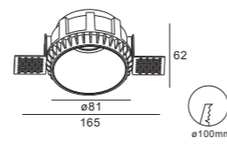
DL0177-G Gu10/Mr16 Downlight Cutout :Ø100mm Optional :ALDL1401 ALDL1373 ALDL1022
