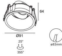
DH0106 Gu10/Mr16 Downlight Cutout :Ø83mm Optional :ALDL1401 ALDL1373 ALDL1022
