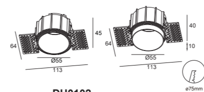
DH0102 Gu10/Mr16 Downlight Cutout :ø75mm Optional :ALDL1401 ALDL1373 ALDL1022
