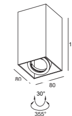
CH0179 Gu10/Mr16 Downlight CE, I, IP20
