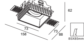
DH0035 Gu10/Mr16 Downlight Cutout :85X85mm Optional :ALDL1401 ALDL1373 ALDL1022
