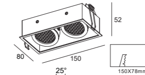
DH0094 Gu10/Mr16 Downlight Cutout :150X78mm
