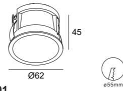
DH0101 Gu10/Mr16 Downlight Cutout :ø55mm Optional :ALDL1401 ALDL1373 ALDL1022
